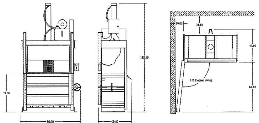
V63 with 6 x 48 Cylinder
